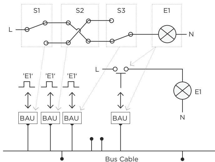
Figure 2. Converting a conventional system into a bus system
