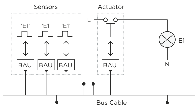
Figure 3. Divided functionality of a bus system
